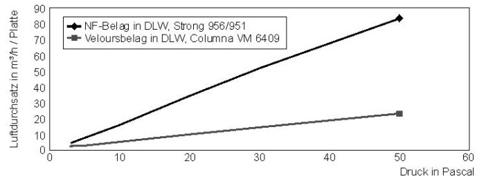
VENTEC H 38 R 15 with covering
