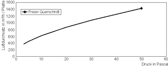
VENTEC H 38 R 15 without covering
